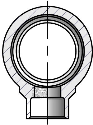
SECTION C-C SCALE 1.50 : 1
